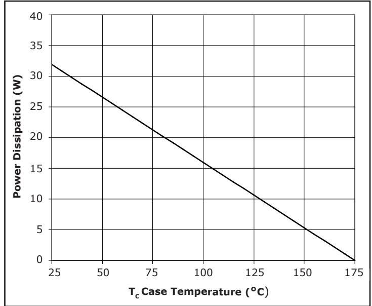
Figure 6. Power Derating
